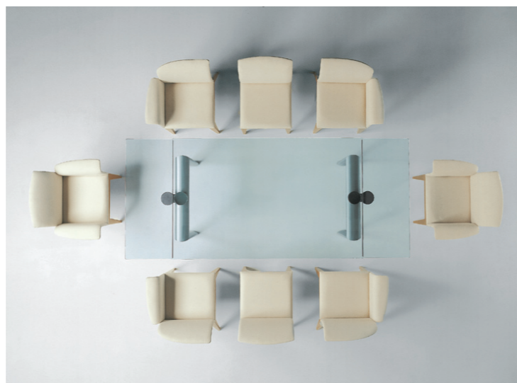
10 Option
